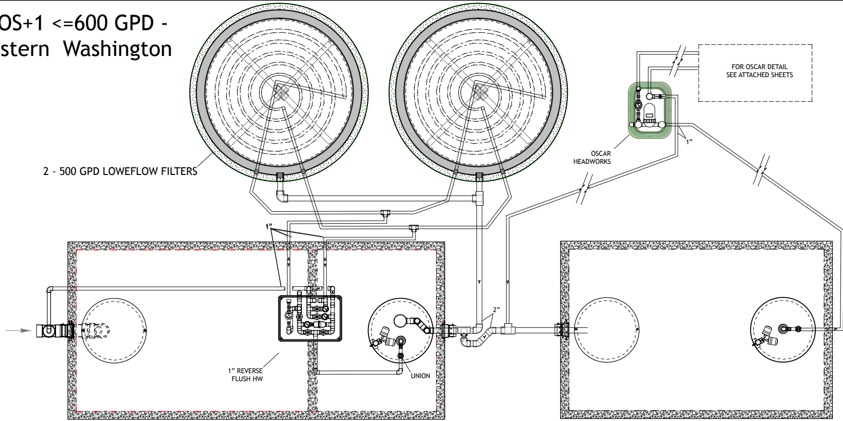
1750 Gallon Pre-cast Concrete Double Compartment Tank
